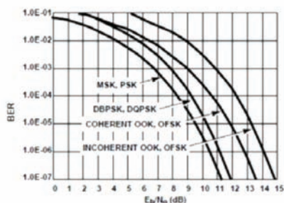
Figure 3. Example of the Relationship BER and Eb/No
