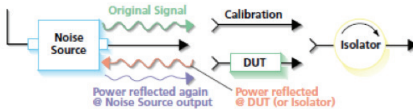
Figure 2: Impedance Mismatch Reflection Illustration
